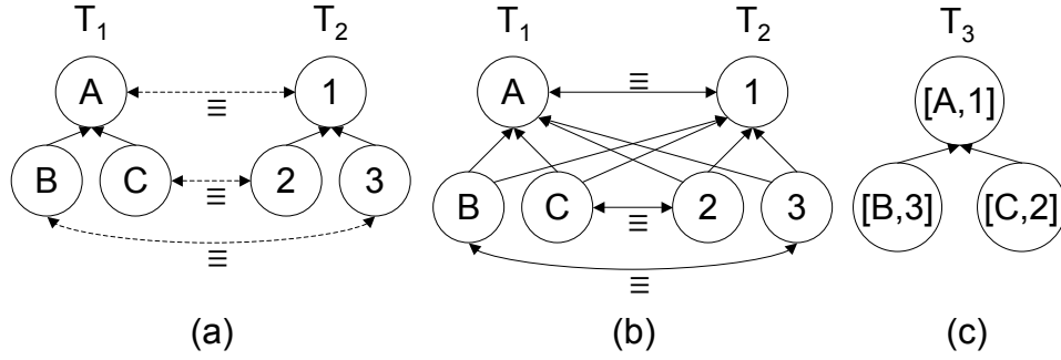
Fig. 4. Merging with and without fusing equivalent taxa.
