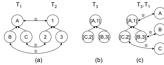
Fig. 2. Projecting Taxonomy 1 from the Merge.
