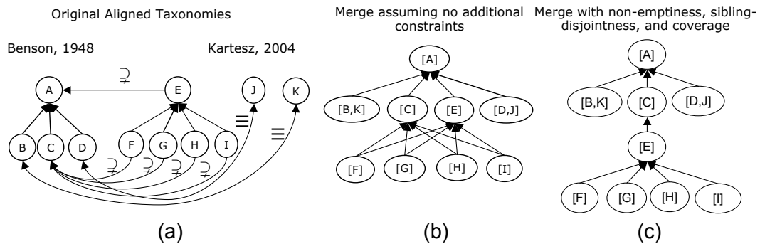
Fig. 6. Merging Ranunculus hispidus under different assumptions. For clarity, the disjointness relations between taxa in (c) are not shown. See text for further detail.
