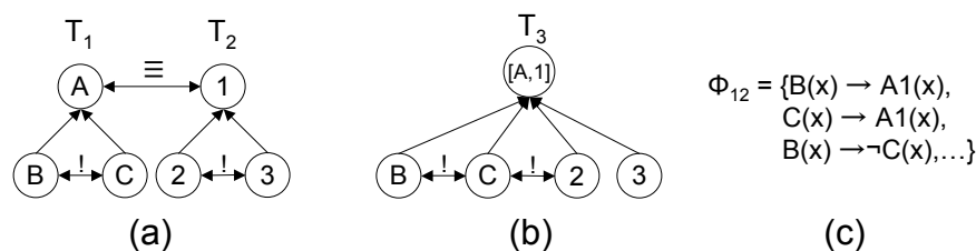
Fig. 1. Given the alignment in (a), the merge in (b) violates all the described desiderata, except for D5 (Closure). The merge in (c) shows a violation of D5.
