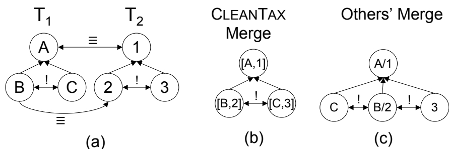
Fig. 8. Comparing merges for the taxonomies in (a) under the parent-coverage constraint. CLEAN TAX correctly merges taxa C and 3 (b) while the others do not (c).
