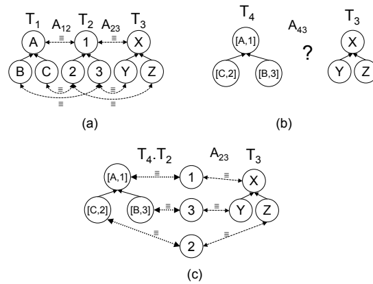
Fig. 3. Using the Projection.
