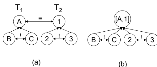
Fig. 7. Constraints placed on taxonomies before the merge may not apply to the result of the merge.
